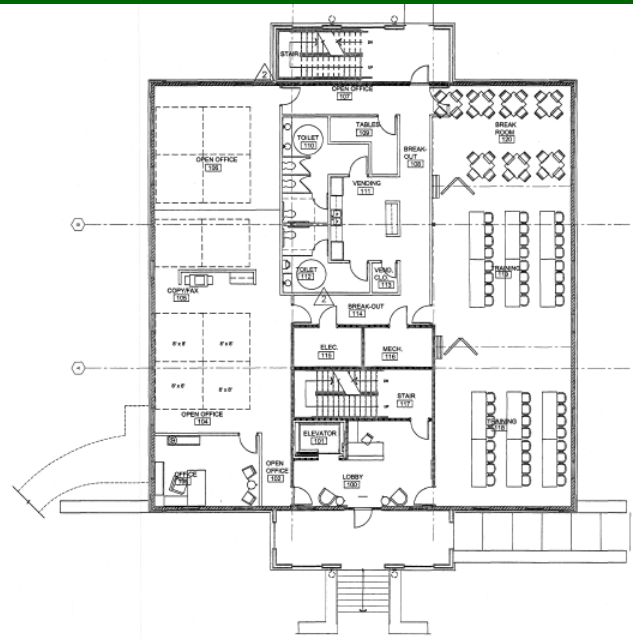
2 CONCEPTUAL SPACE PLAN-FIRST FLOOR
